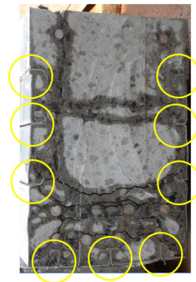
Fig. 10 Beam section by saw-cut
