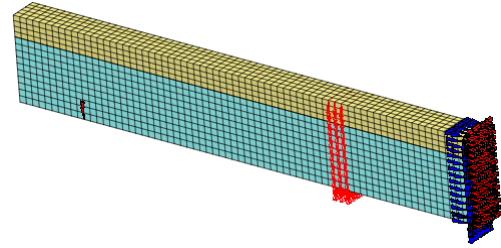
Fig. 19 Concrete model
